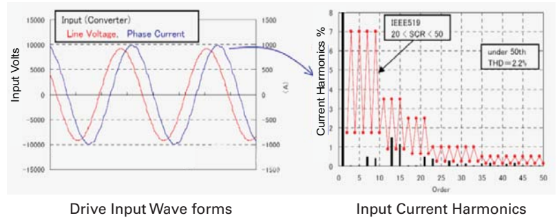
Drive Input Wave forms
